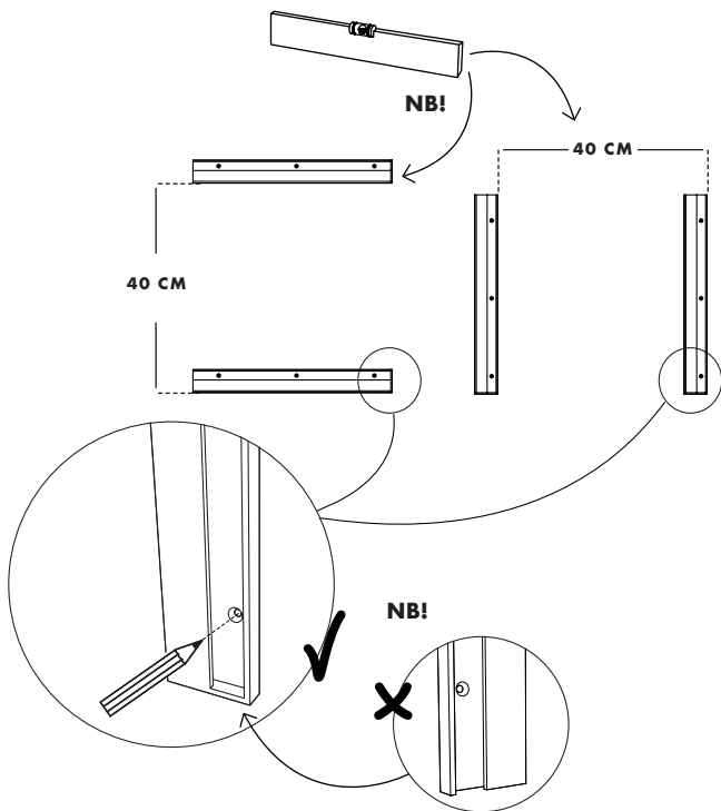
VERTICAL MIRROR
