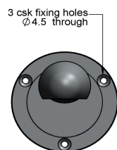
MOUNTING SEAT & ESCUTCHEON COVER Dimensions in mm
