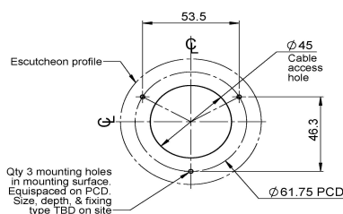
MOUNTING HOLE DETAILS Dimensions in mm
